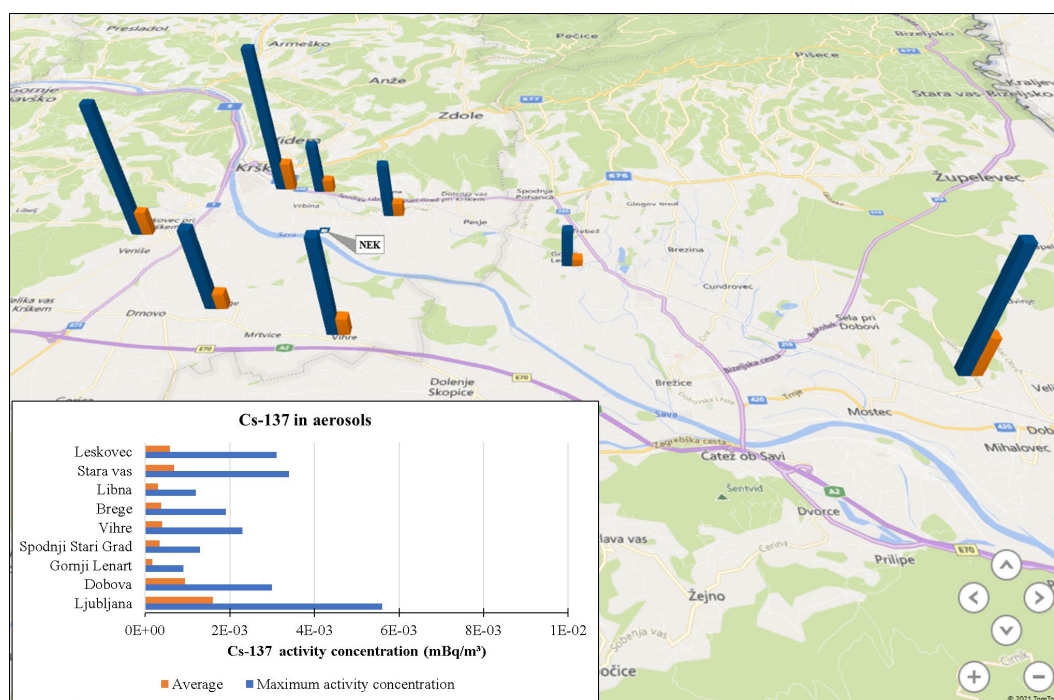
Figure I8: Review of average and highest measured activity concentrations of Cs-137 in air.
