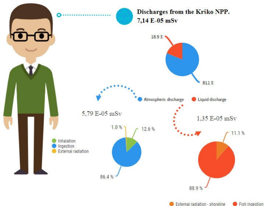
Figure P1: Review of estimated annual effective doses for artificial radionuclides in the framework of environmental radioactivity monitoring in the vicinity of the Krško NPP in 2020
