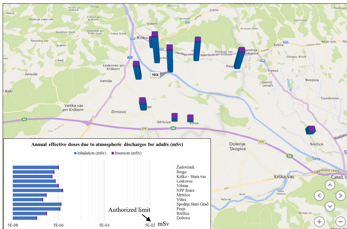
Figure P3: Review of estimated annual effective doses for artificial radionuclides for air emissions in the vicinity of the Krško NPP in 2020
