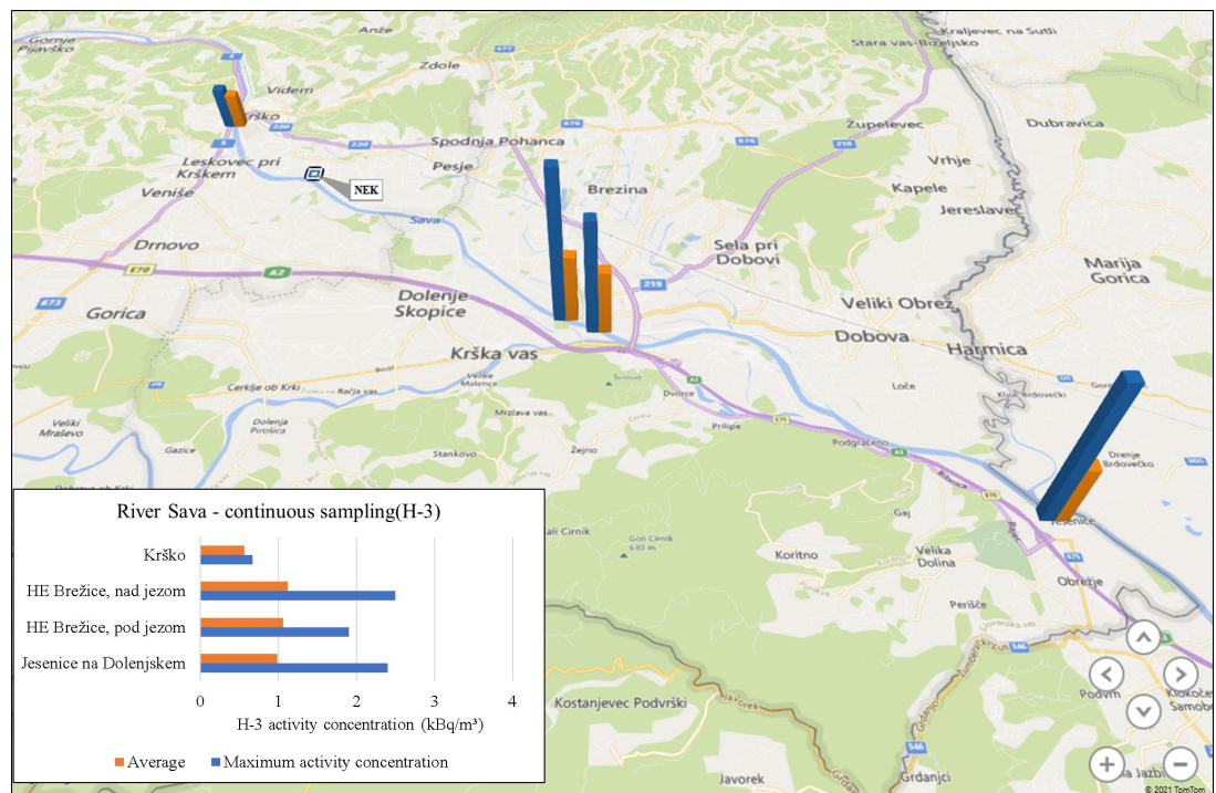
Figure I1: Overview of average and highest measured activity concentrations of H-3 in the Sava River at stations with continuous sampling mode upstream and downstream of the Krško NPP dam in 2020. The long-term average (since 2002) of monthly activity concentrations of H-3 activity in Brežice is 4.0 kBq/m³. The long-term average (since July 2017) of the monthly activity concentrations of H-3 at the sampling station in front of the Brežice HPP dam is 2.9 kBq/m³. Activity concentrations of tritium in Sava at Jesenice na Dolenjskem sampling station are lower due to additional dilution of the Sava with Krka and Sotla. The long-term average of monthly concentrations of H-3 activity in Jesenice na Dolenjskem is 2.4 kBq/m³.
