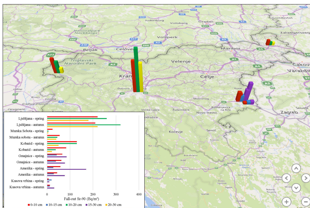
Figure I12: Fallout of Sr-90 in Slovenia (Ljubljana, Murska Sobota, Kobarid) and in the vicinity of the Krško NPP (Gmajnice, Amerika, Kusova vršina) in 2020
