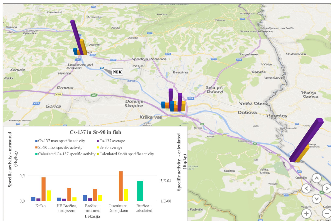
Figure I4: Specific activities of Cs-137 and Sr-90 in fish samples in 2020
