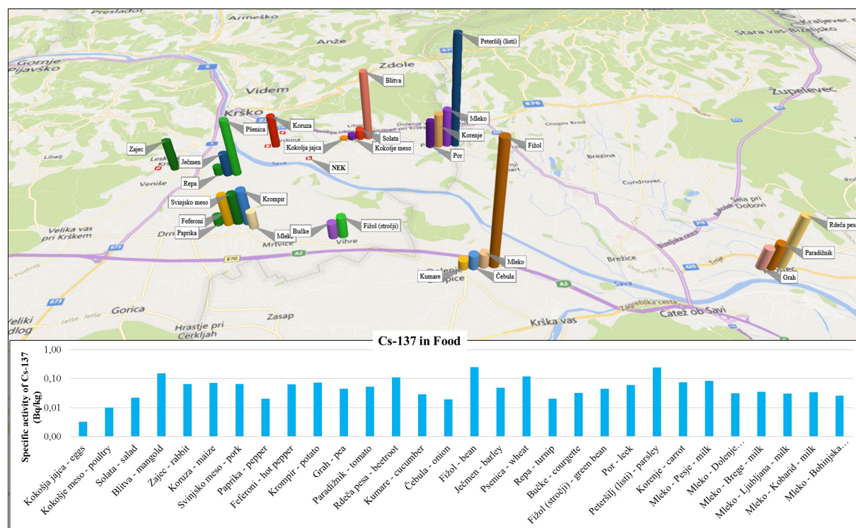
Figure I13: Specific activities of Cs-137 in food in the vicinity of the Krško NPP in 2020
