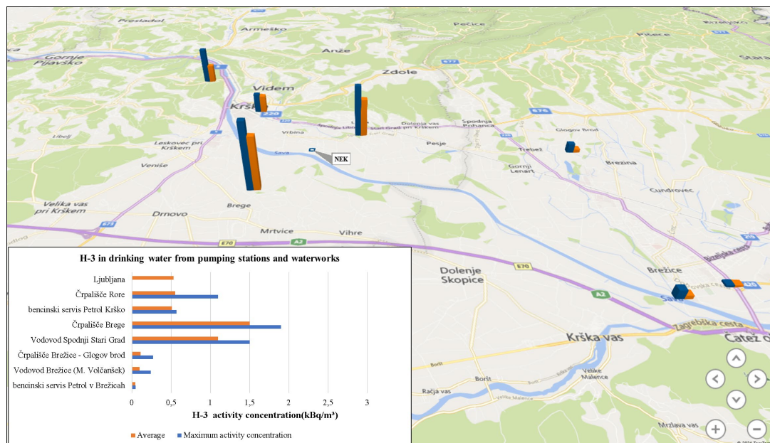
Figure I5: Review of average and highest measured activity concentrations of H-3 in drinking water from pumping stations and waterworks in the municipalities of Krško and Brežice at locations where they are sampled continuously or quarterly.
