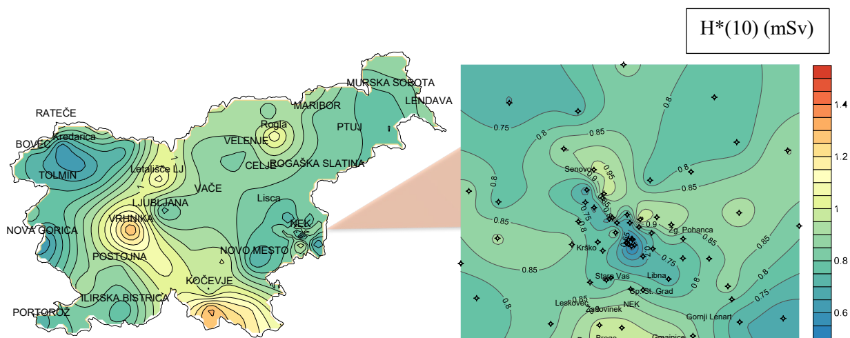
Figure I10: Average annual ambient dose equivalent H^*(10) in Slovenia and in the vicinity of the Krško NPP in 2020
