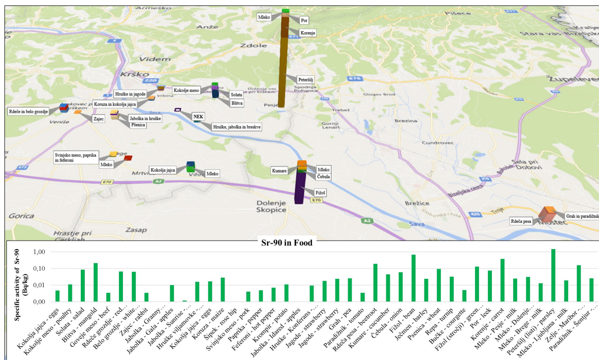
Figure I14: Specific activities of Sr-90 in food in the vicinity of the Krško NPP in 2020.
