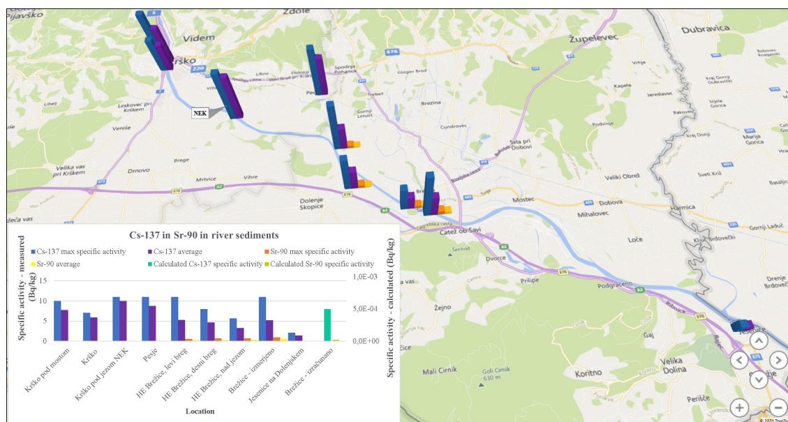
Figure I3: Specific activities of Cs-137 and Sr-90 in river sediments in 2020
