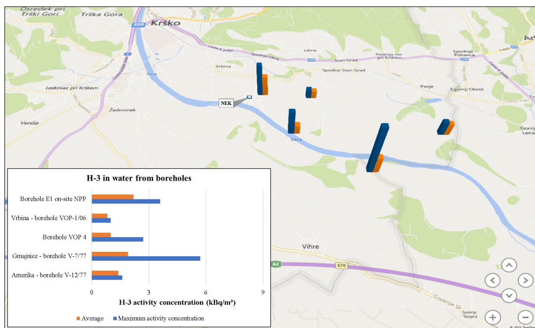
Figure I6: Review of average and highest measured activity concentrations of H-3 activity in water from the boreholes.
