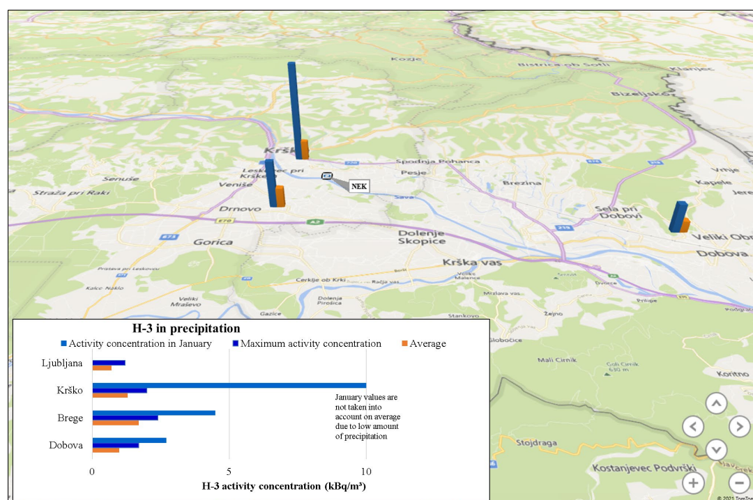
Figure I7: Review of average and highest measured activity concentrations of H-3 in precipitation
