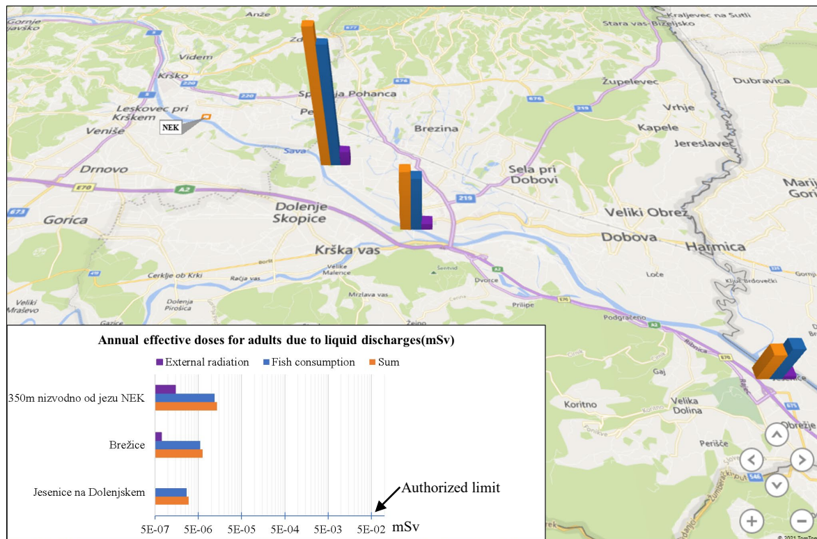
Figure P2: Review of estimated annual effective doses for artificial radionuclides for liquid discharges from the Krško NPP in 2020.
