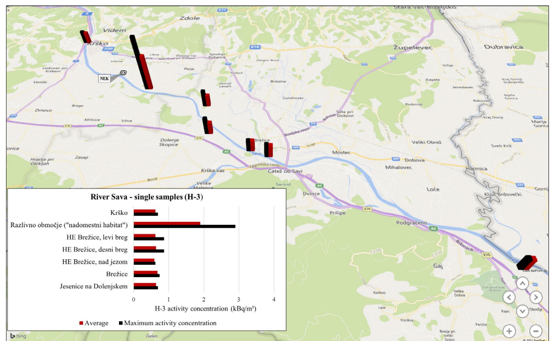
Figure I2: Review of average and highest measured activity concentrations of H-3 in the Sava River at locations upstream and downstream of the Krško NPP dam, where single (monthly or quarterly) samples are collected.
